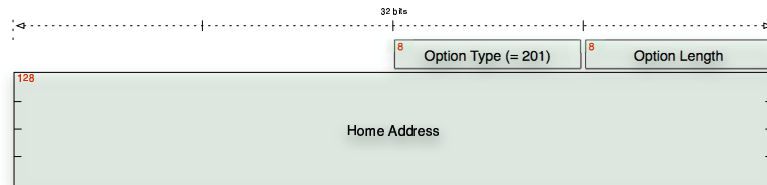
Fig. 11. Home Address Option (HAO)
